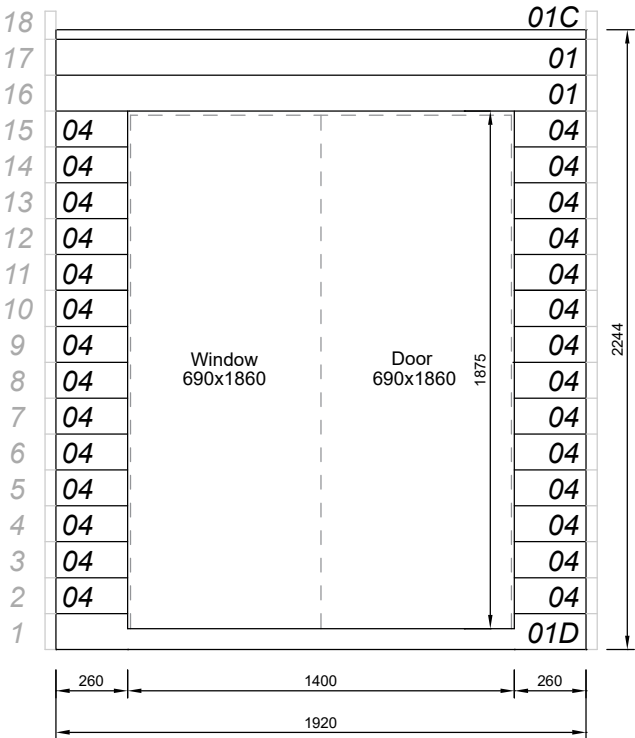
Wall 2 (front) View from the outside
