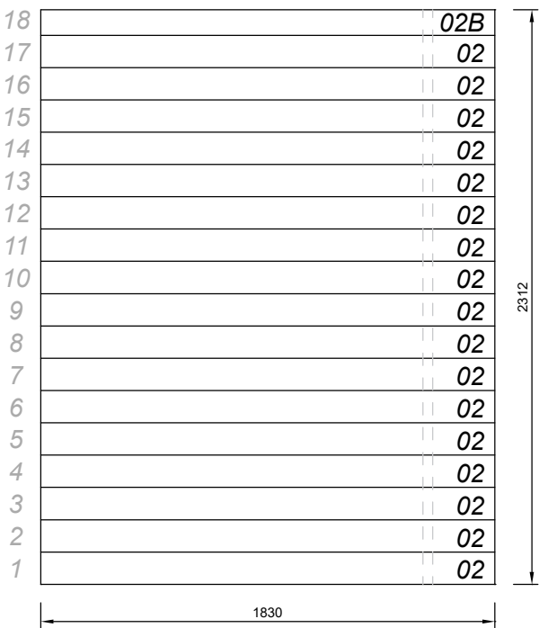
Wall A (left) View from the outside
